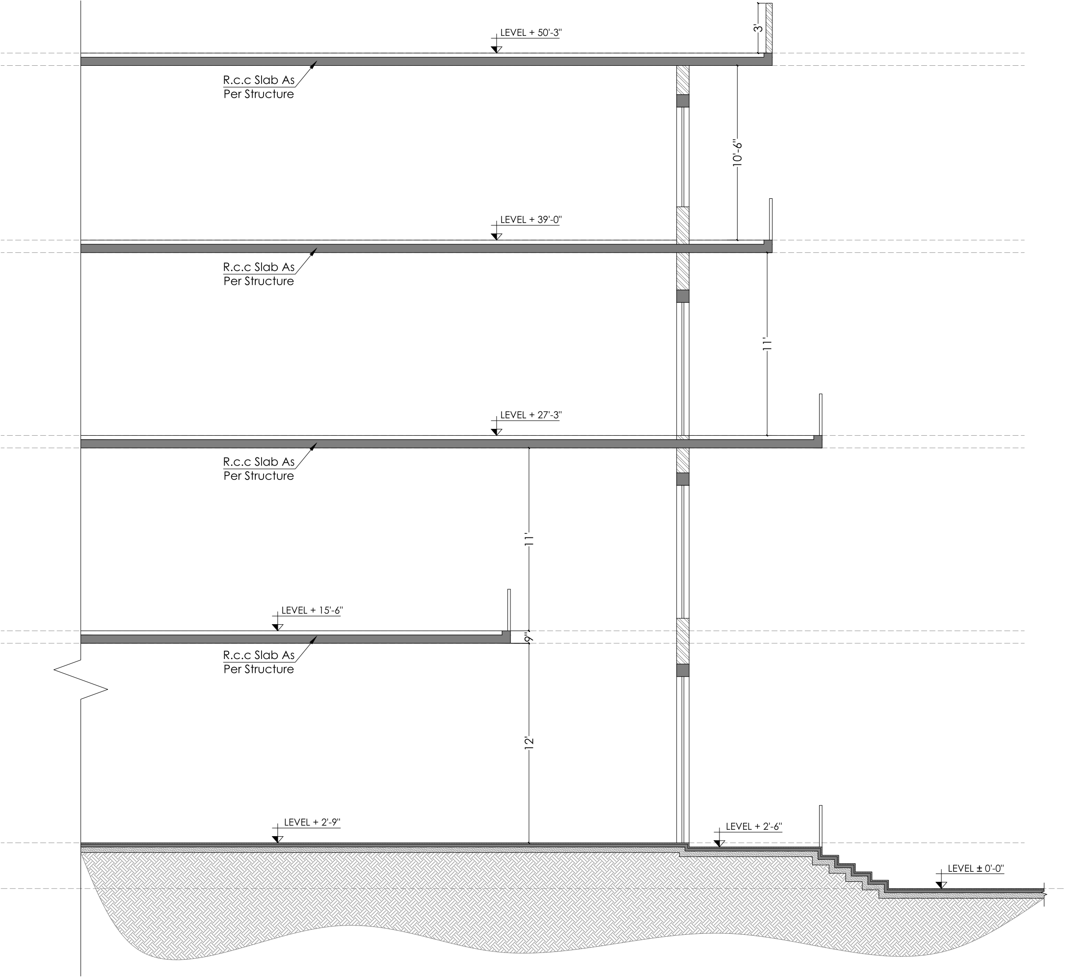
PART SECTION
